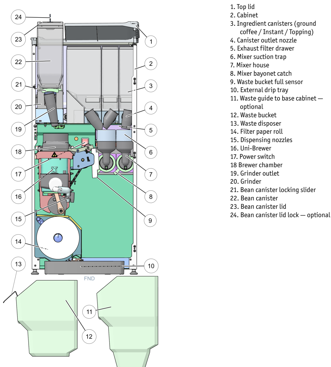
Inside view Unibrewer (small model)
